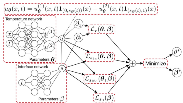
Fig. 11 Two-phase Stefan problem: PINN architecture for inferring the latent temperature fields u_1(x, t) , u_2(x, t) , and phase-transition interface s(t) , from scattered noisy observations of temperature
