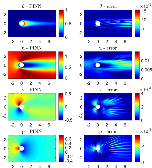
Fig. 5 Forced convection of flow past a cylinder with constant temperature surface: temperature, velocity and pressure fields inferred by PINN with sensor configuration Case 3 (left) and the pointwise absolute errors between CFD and PINN (right)
