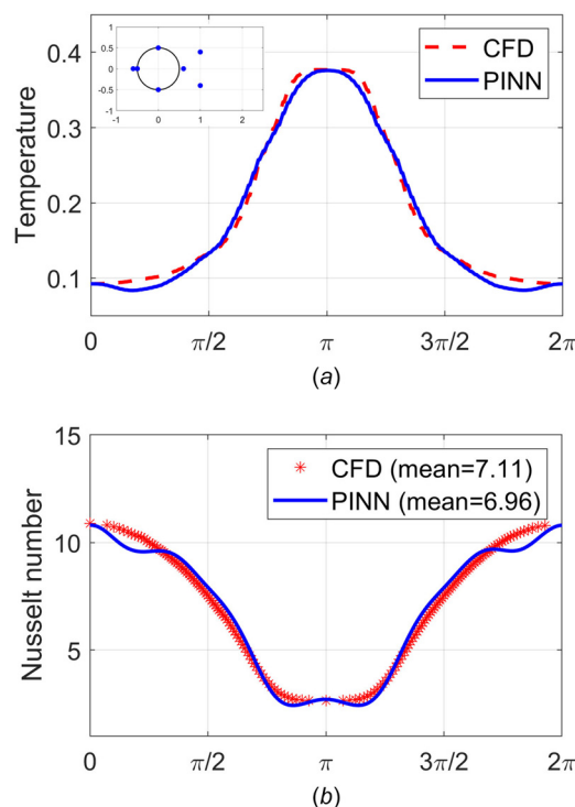
Fig. 7 Forced convection of flow past a cylinder with constant flux surface: (a) temperature and (b) Nusselt number profiles on the cylinder boundary. The sensor configuration is given at the top-left corner. With this setup, the errors of (\theta, u, v, p) inferred by PINN are 3.18%, 0.18%, 0.24%, and 0.46%, respectively.
