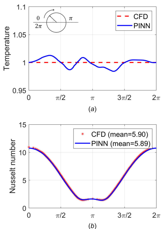
Fig. 6 Forced convection of flow past a cylinder with constant temperature surface: (a) temperature and (b) Nusselt number profiles on the cylinder boundary, inferred by PINN with sensor configuration Case 3
