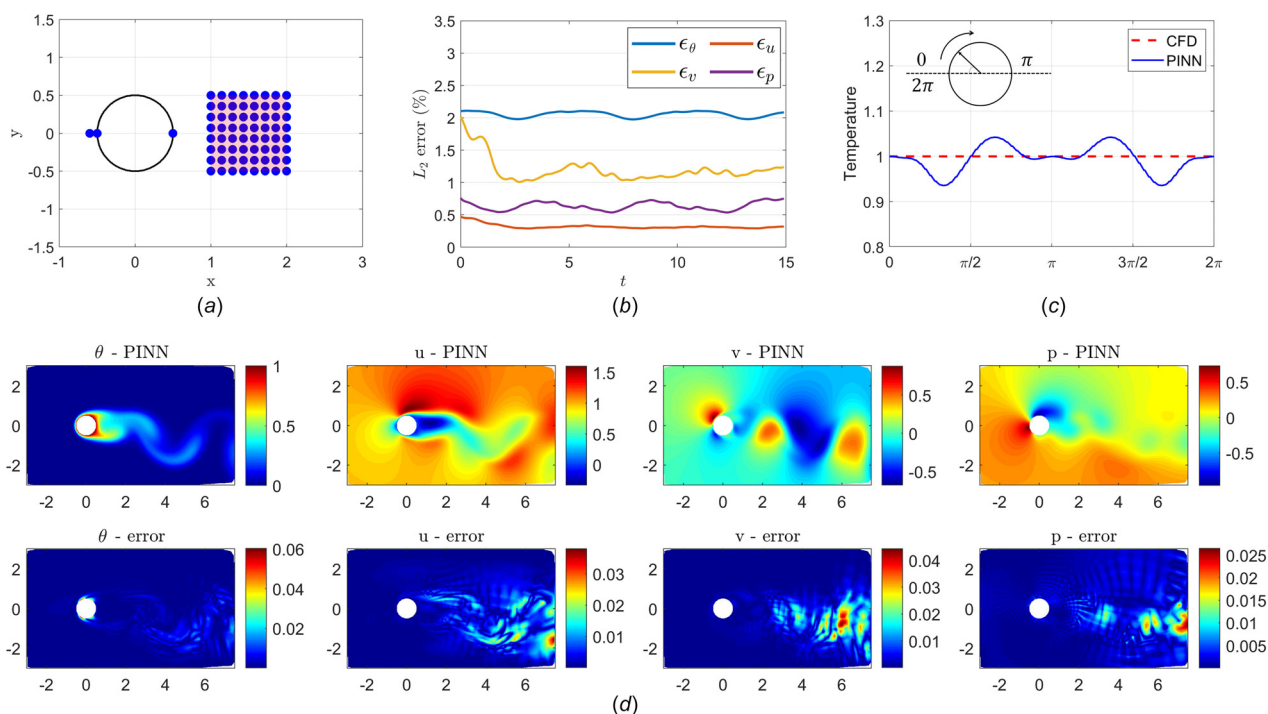
Fig. 10 Mixed convection of flow past a cylinder. (a) Temperature measurements. DPIT measures temperature in an area represented by a red rectangle with 8 \times 8 grids. (b) The relative L_2 -norm errors of temperature, velocity, and pressure fields along time inferred by PINN. (c) The mean temperature profile on the cylinder surface. (d) The 2D fields at t = 5.0 inferred by PINN and the corresponding pointwise error maps.
