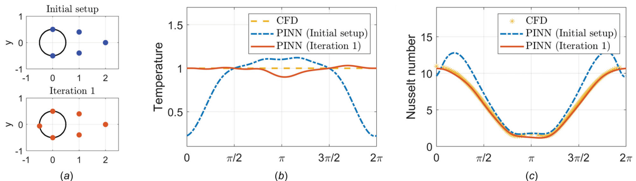
Fig. 9 Active sensor placement: (a) the sensor configurations of initial setup and after the first iteration, (b) temperature profile on the cylinder surface, and (c) Nusselt number on the cylinder surface
