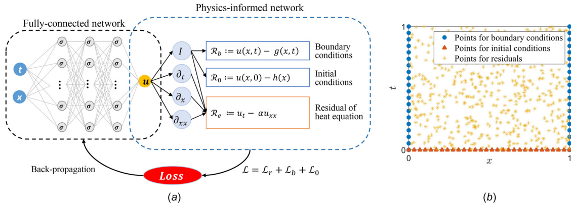
Fig. 1 Overview of physics-informed neural networks (PINNs). (a) Schematic of PINN framework. A fully connected neural network is used to approximate the solution u(x, t) , which is then applied to construct the residual loss \mathcal{L}_r , boundary conditions loss \mathcal{L}_b and initial conditions loss \mathcal{L}_0 . The derivatives of u are computed by automatic differentiation in TensorFlow [26]. The parameters of the fully connected network are trained using gradient-descent methods based on the back-propagation of the loss function. (b) Schematic of point selection for PINN in the computational domain. The points with different colors correspond to different terms in the loss function. Note that the residual points for computing the residual loss can be randomly selected in the space-time domain.
