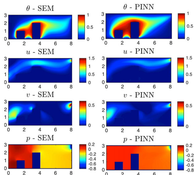
Fig. 3 Forced convection in an enclosure: comparison of \theta , u , v , and p inferred by PINN and the reference simulation results by the spectral element method
