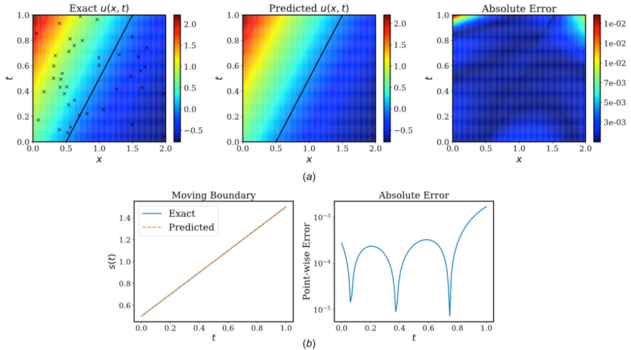
Fig. 12 Inverse two-phase Stefan problem: (a) exact temperature solution along with training data (x) versus the predicted solution. The relative L^2 error: 2.57 \times 10^{-3} . (b) Left: comparison of the predicted and exact predicted moving boundary. Right: the absolute error between the exact and the predicted free boundary for t \in [0, 1] . The L^2 error is 3.93 \times 10^{-4} .
