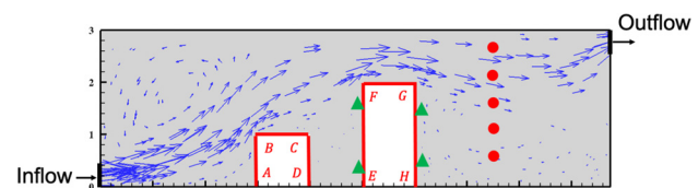
Fig. 2 Forced convection in an enclosure. The boundaries in red color are at higher temperature, and the cooling inflow enters from the left-bottom and exits at the right-top. The blue arrows show the velocity vectors. The temperature at the boundaries EF and GH are not known. The green triangles represent the temperature probes while the red circles denote the velocity probes.
