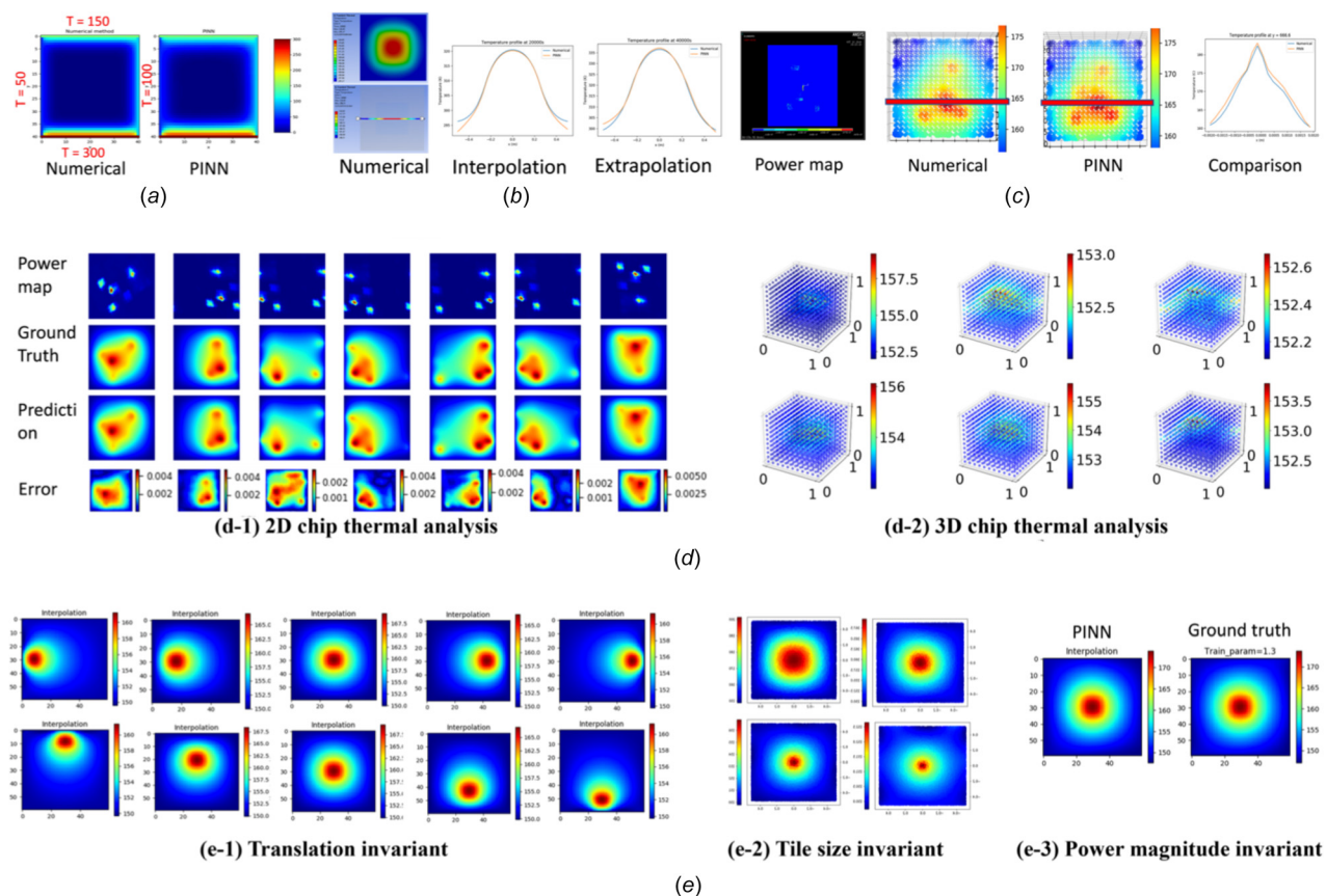
Fig. 14 Solving the heat equation on electronic chips. (a) 2D transient heat transfer problem with Dirichlet boundary conditions; (b) 2D transient heat transfer problem with heat source at the center of the square. Comparisons are made on the horizontal centerline within the training time zone (interpolation) and beyond the training time zone (extrapolation). (c) 2D heat transfer on a chip. Comparisons are performed on the red section lines passing through the hottest spot on chip. (d) Thermal analysis for 2D and 3D chips using PINN-inspired Auto-Encoder Image Gradient based approach [22]. (e) Temperature prediction on a chip with a single tile as power source by a parameterized PINN, for different power source locations, tile sizes with power, and power magnitudes. (Courtesy of the Central ML ANSYS team.)
