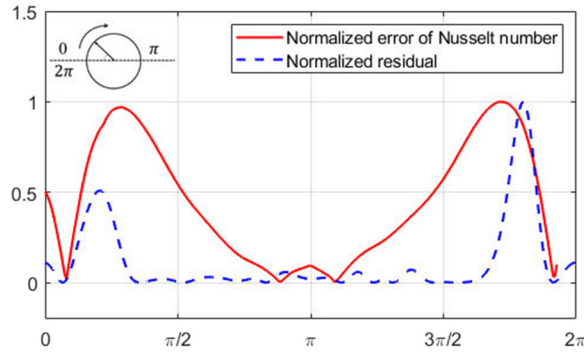
Fig. 8 Active sensor placement: the normalized error of Nusselt number and the normalized residual of the heat equation on the cylinder surface, inferred by PINN with sensor configuration Case 1 in Fig. 4. We can observe the correlation between the two profiles.
